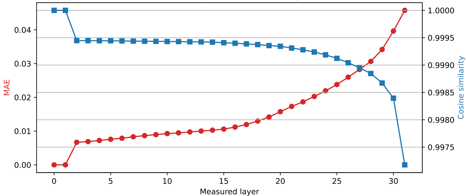
Mistral-7B-Instruct-v0.3 | Quantized layer 1 | float32 → int8
