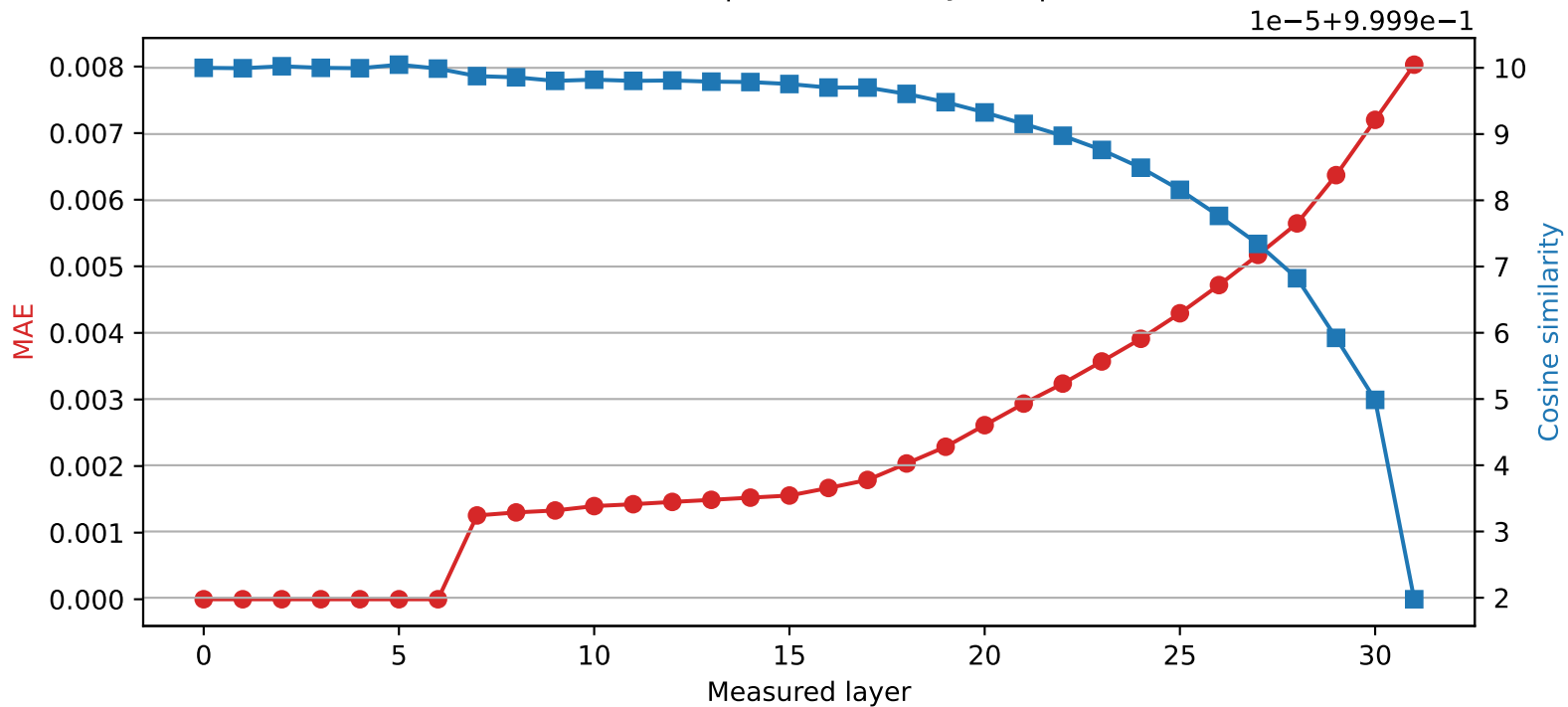
Mistral-7B-Instruct-v0.3 | Quantized layer 6 | float32 → int8
