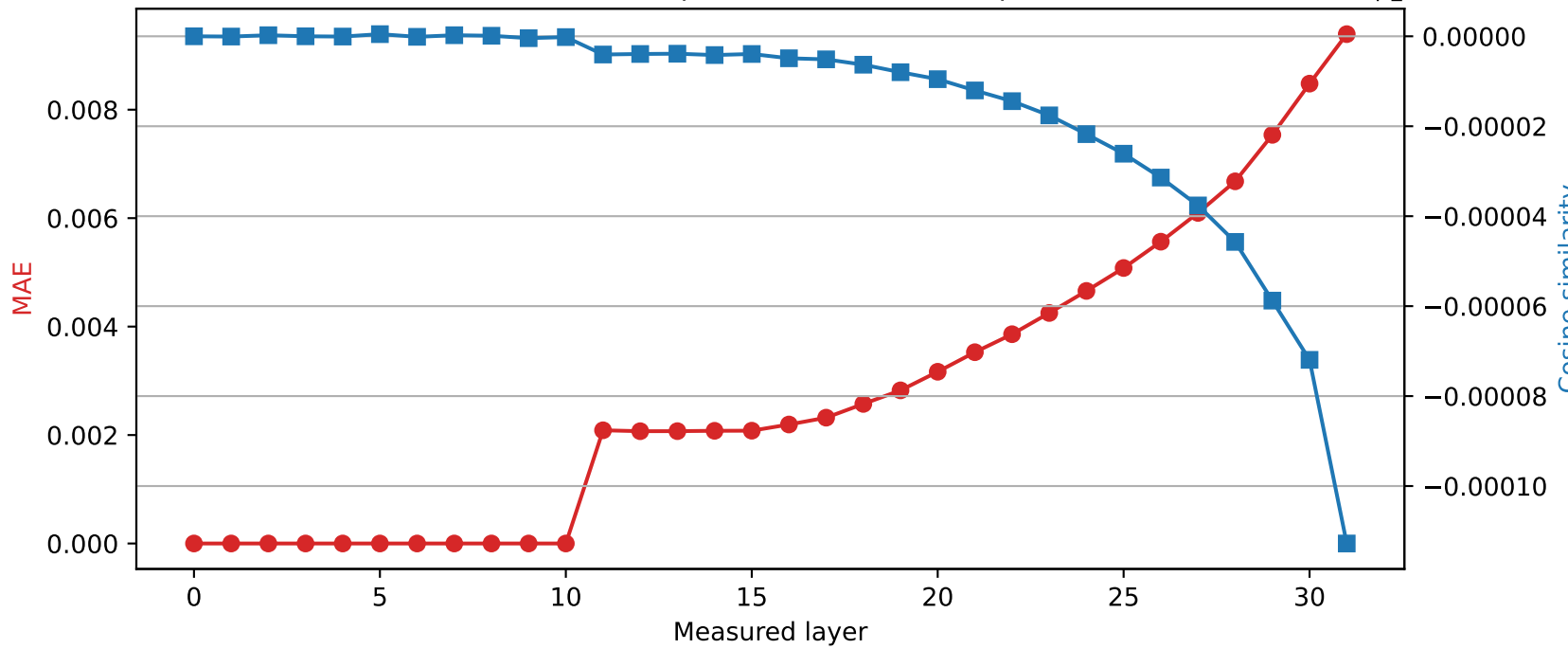
Mistral-7B-Instruct-v0.3 | Quantized layer 10 | float32 \rightarrow int8
