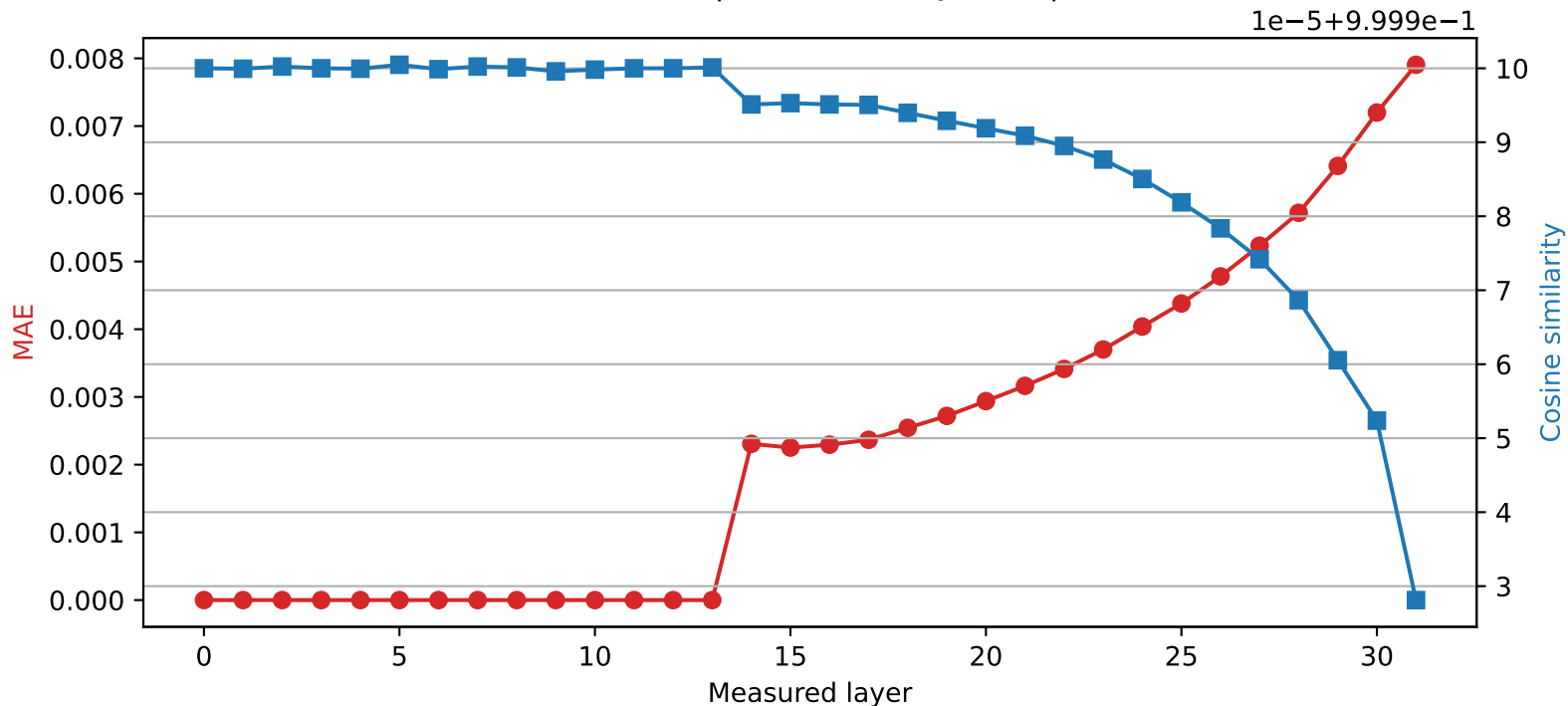
Mistral-7B-Instruct-v0.3 | Quantized layer 13 | float32 \rightarrow int8
