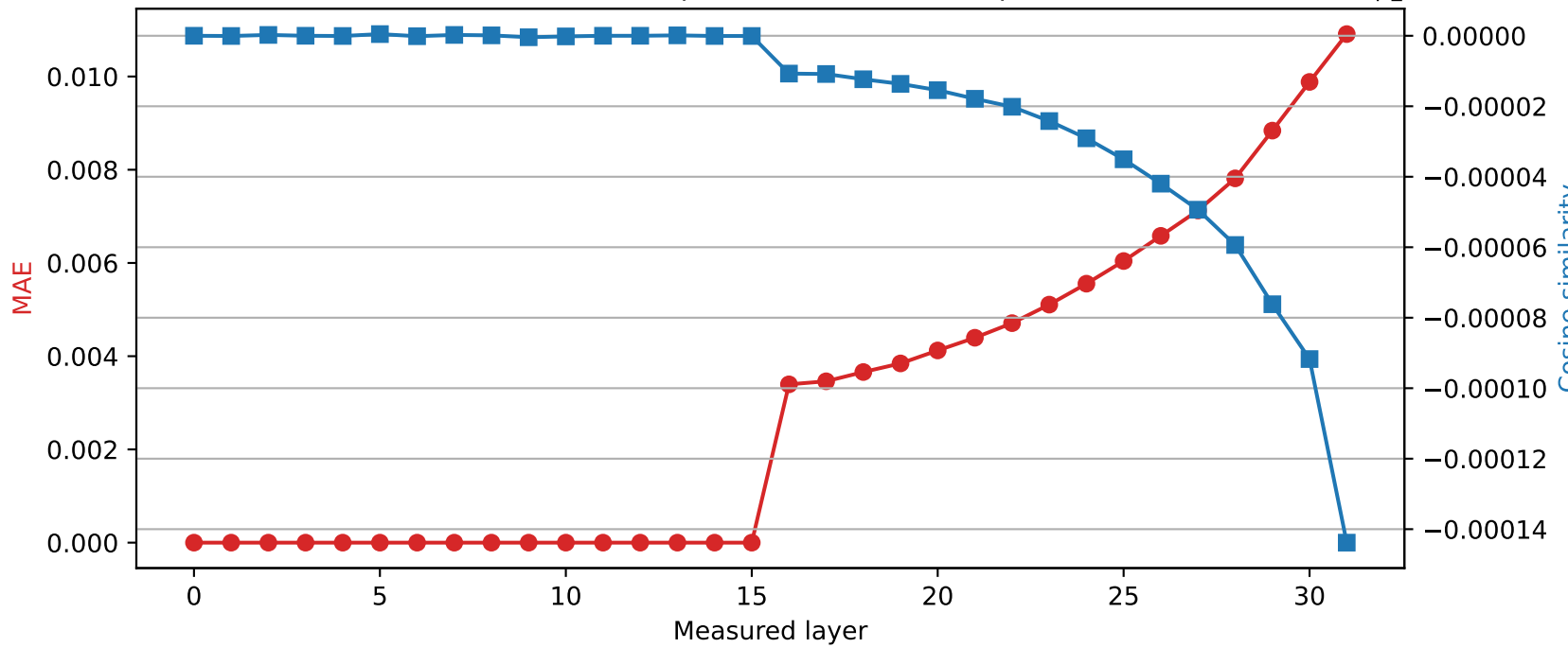
Mistral-7B-Instruct-v0.3 | Quantized layer 15 | float32 \rightarrow int8
