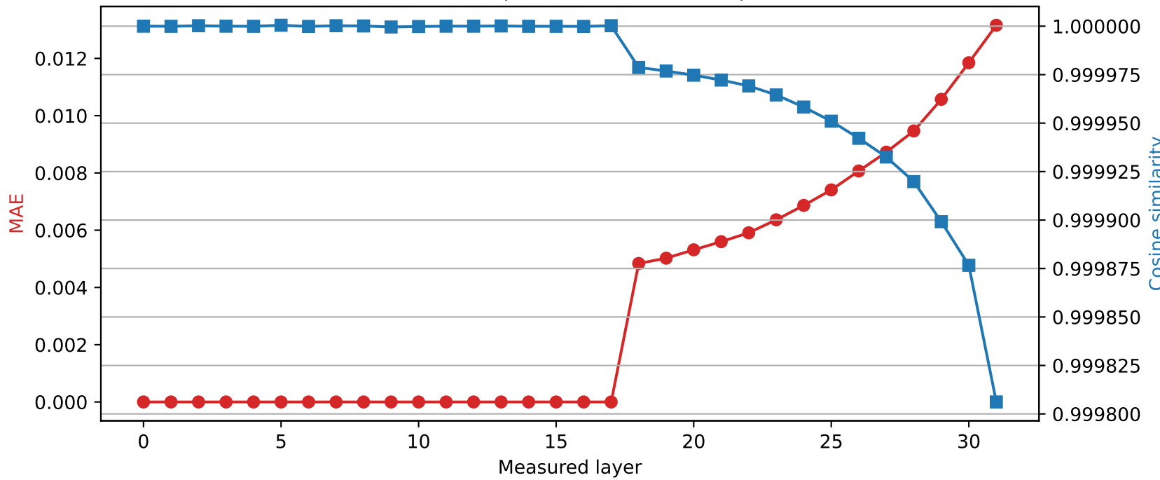
Mistral-7B-Instruct-v0.3 | Quantized layer 17 | float32 \rightarrow int8
