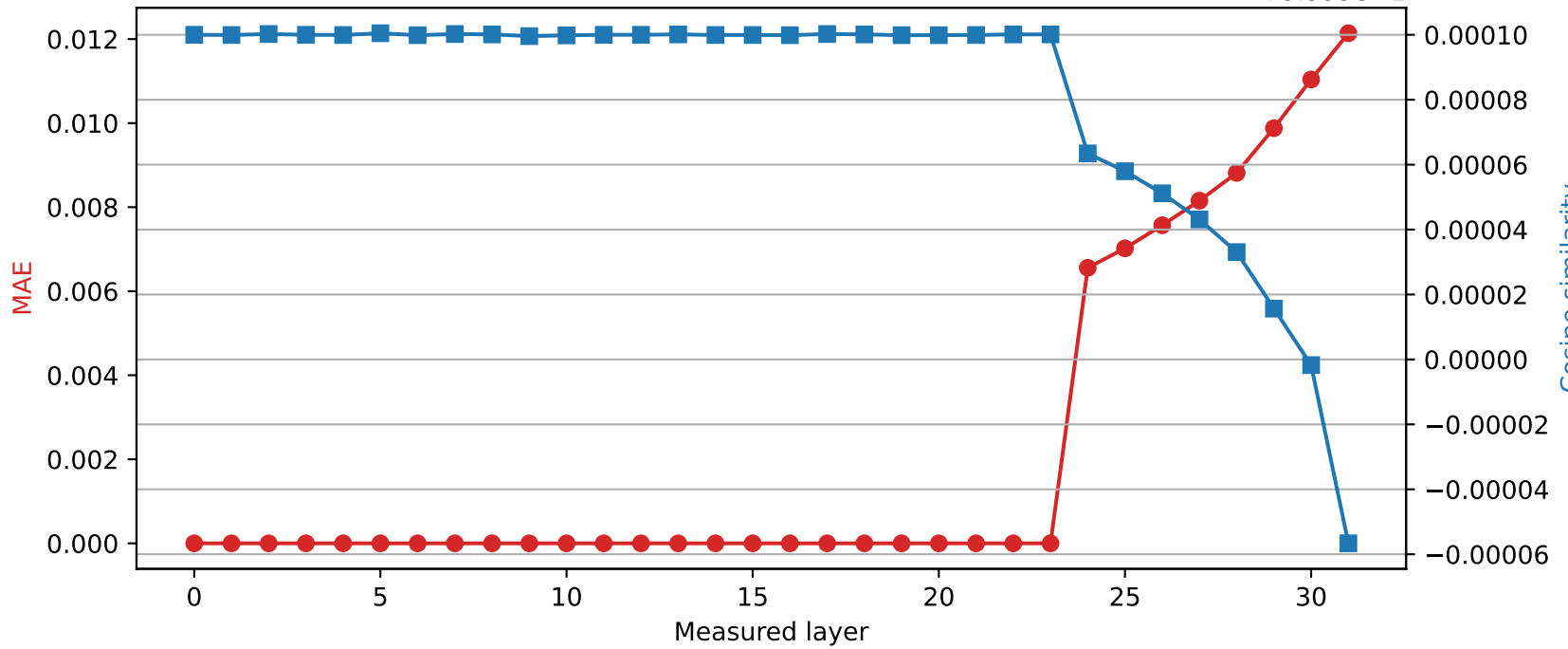
Mistral-7B-Instruct-v0.3 | Quantized layer 23 | float32 \rightarrow int8 +9.999e-1
