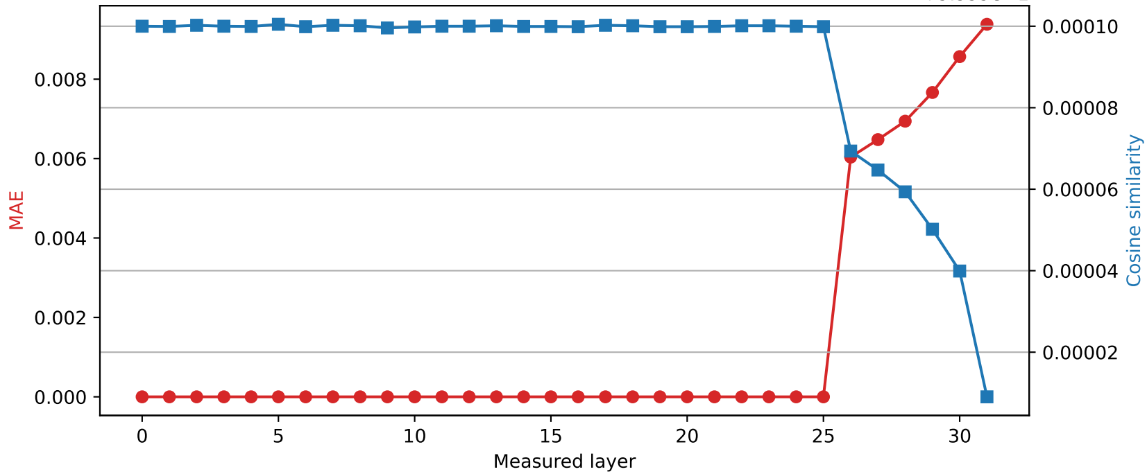
Mistral-7B-Instruct-v0.3 | Quantized layer 25 | float32 \rightarrow int8 +9.999e-1
