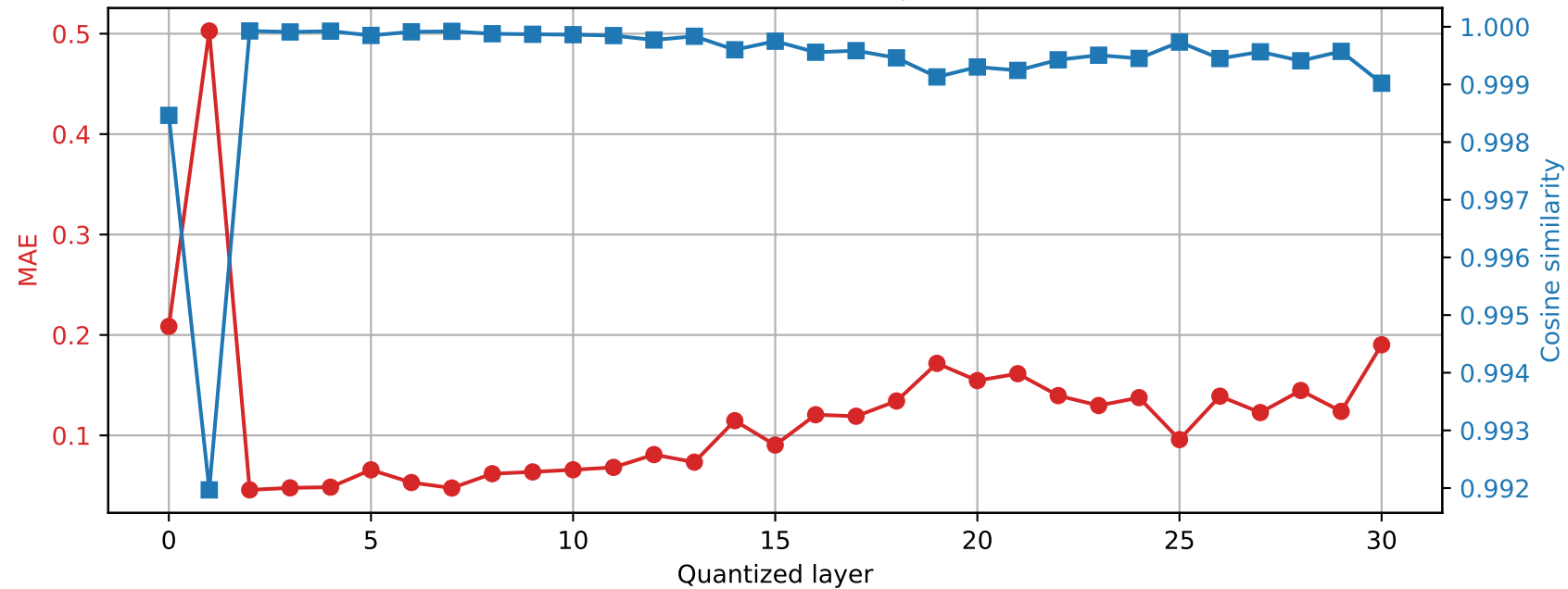
Mistral-7B-Instruct-v0.3 | Prompt 2 Final RMSNorm output damage | float32 → int8
