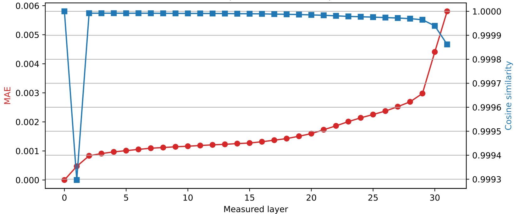
Mistral-7B-Instruct-v0.3 | Quantized layer 0 | float32 → int8
