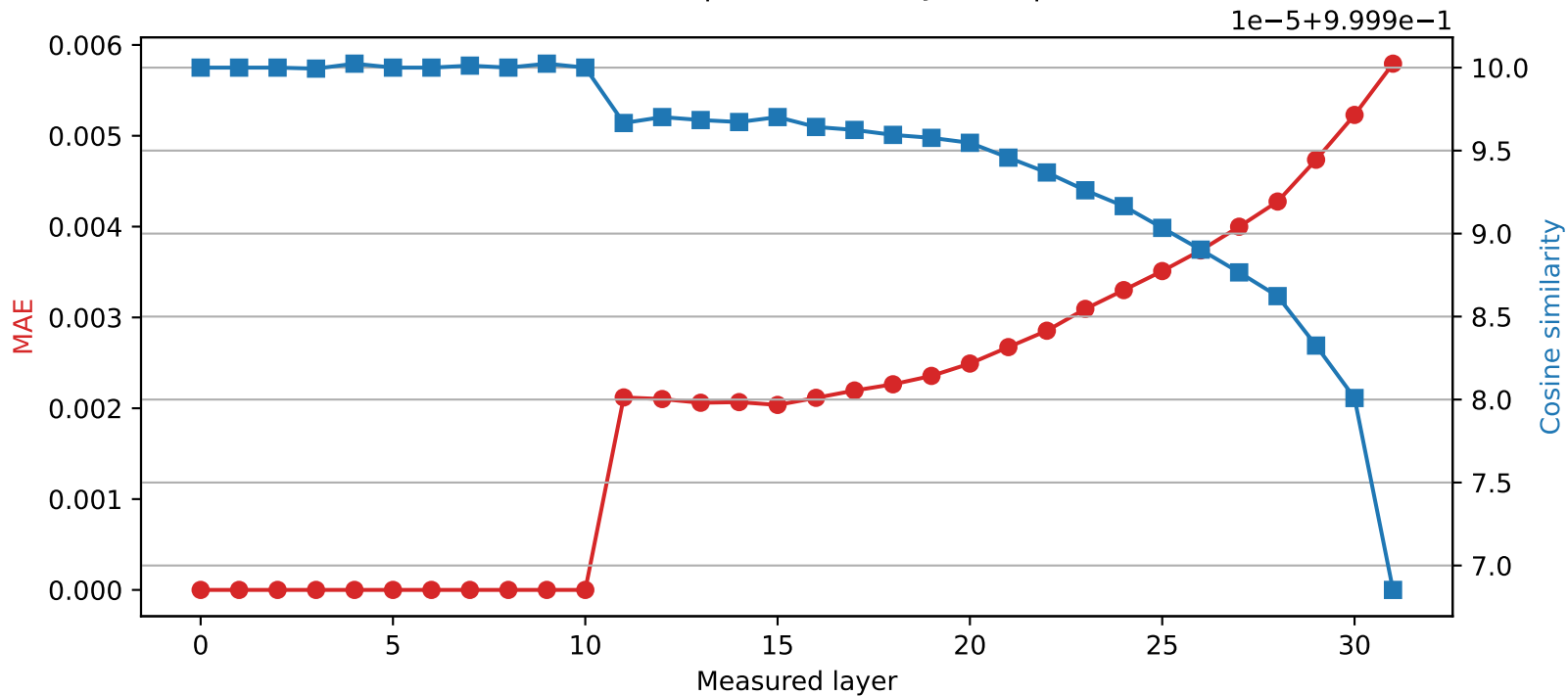
Mistral-7B-Instruct-v0.3 | Quantized layer 10 | float32 \rightarrow int8
