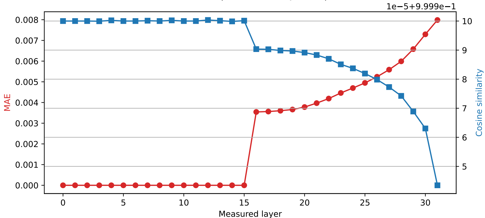
Mistral-7B-Instruct-v0.3 | Quantized layer 15 | float32 \rightarrow int8
