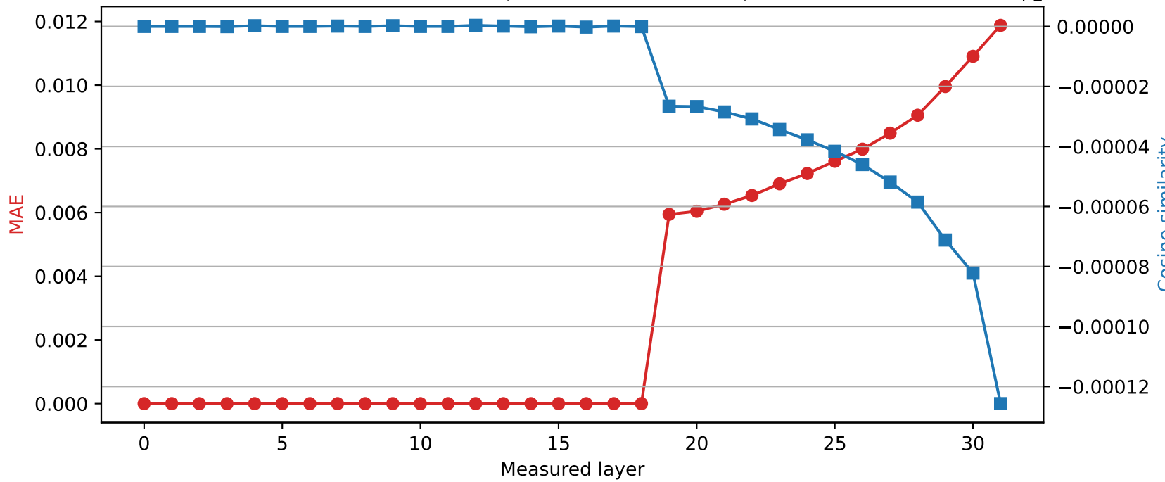
Mistral-7B-Instruct-v0.3 | Quantized layer 18 | float32 \rightarrow int8
