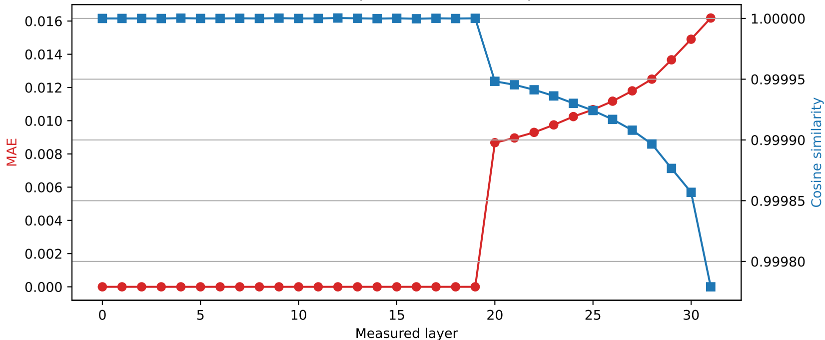
Mistral-7B-Instruct-v0.3 | Quantized layer 19 | float32 \rightarrow int8
