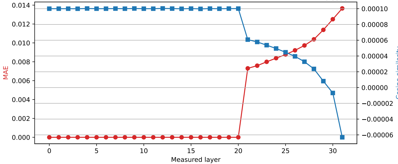
Mistral-7B-Instruct-v0.3 | Quantized layer 20 | float32 \rightarrow int8 +9.999e-1
