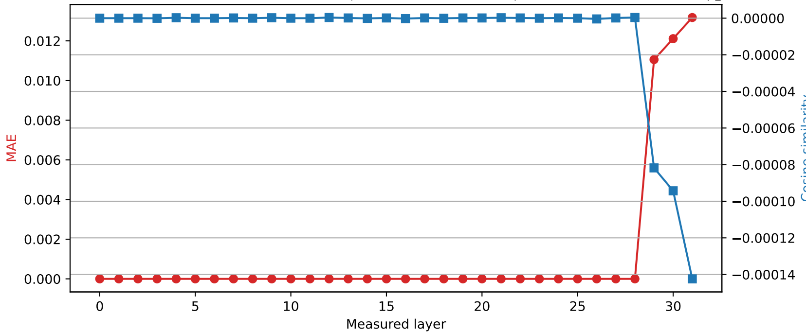
Mistral-7B-Instruct-v0.3 | Quantized layer 28 | float32 \rightarrow int8
