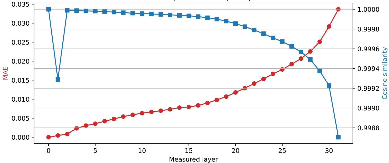
Mistral-7B-Instruct-v0.3 | Quantized layer 0 | float32 \rightarrow int8
