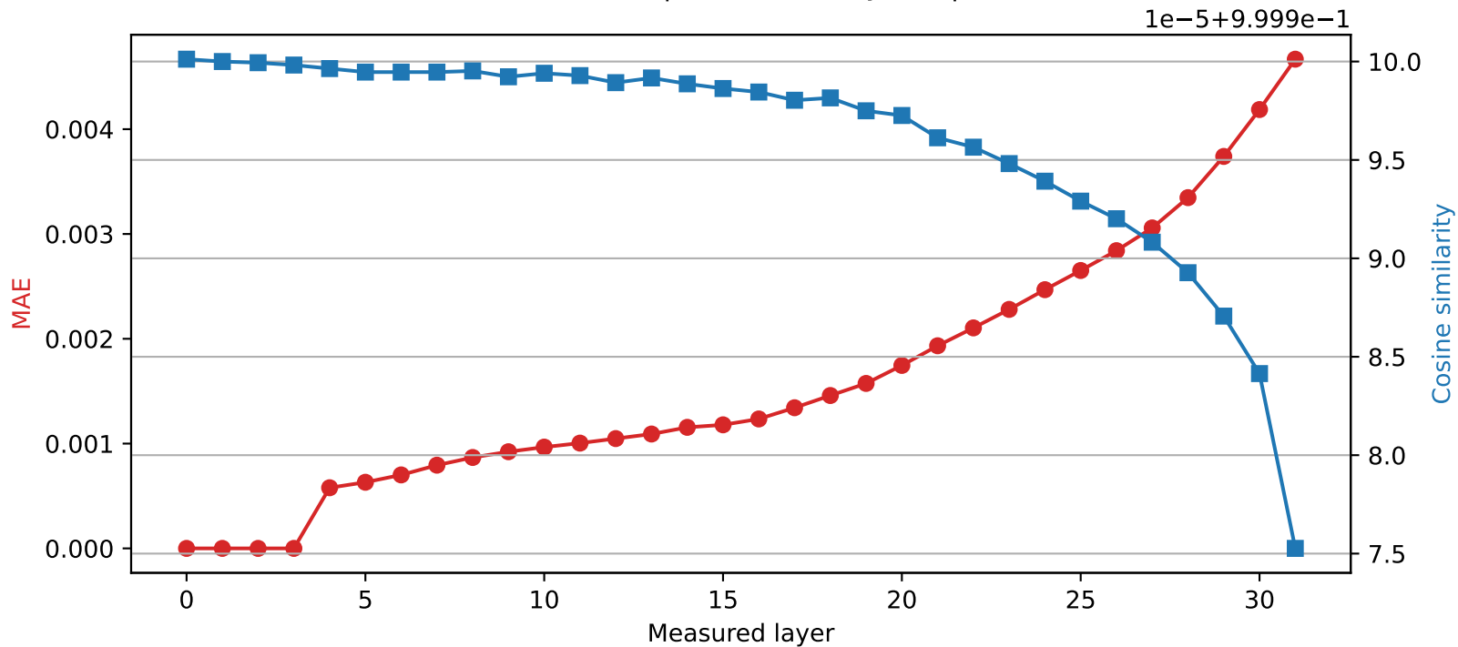
Mistral-7B-Instruct-v0.3 | Quantized layer 3 | float32 → int8
