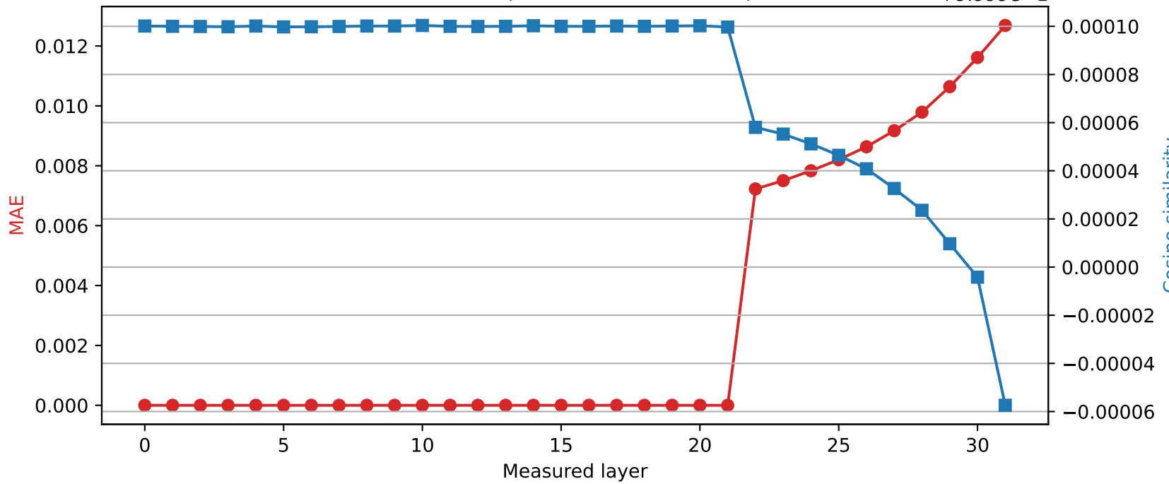
Mistral-7B-Instruct-v0.3 | Quantized layer 21 | float32 \rightarrow int8 +9.999e-1
