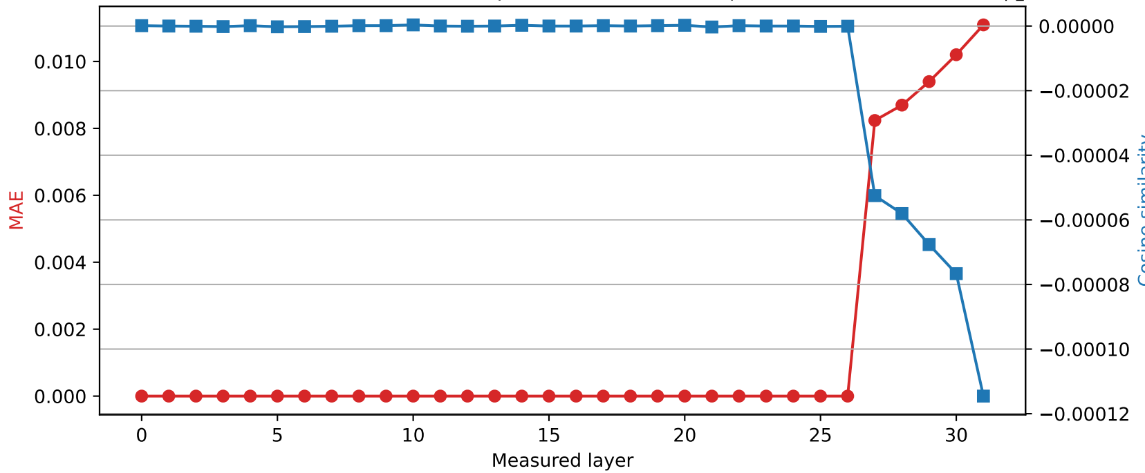
Mistral-7B-Instruct-v0.3 | Quantized layer 26 | float32 \rightarrow int8
