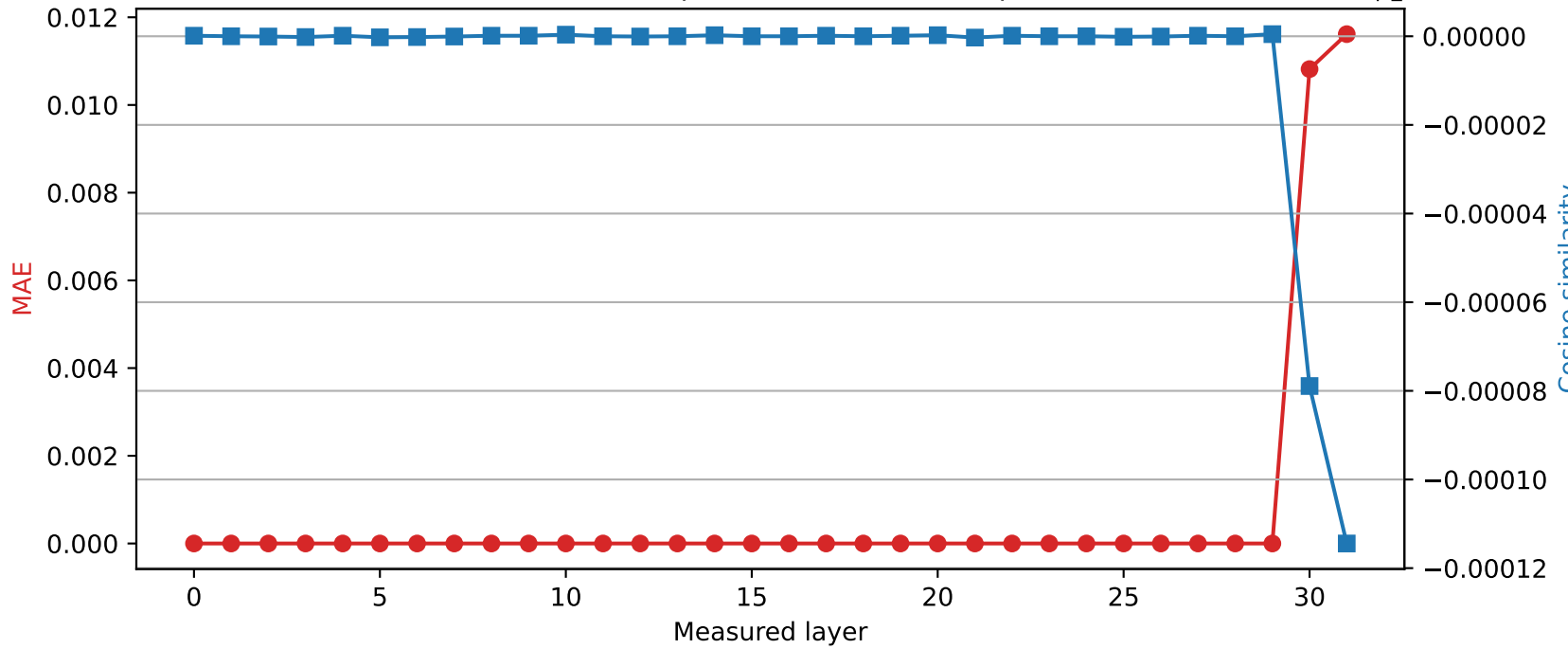
Mistral-7B-Instruct-v0.3 | Quantized layer 29 | float32 \rightarrow int8
