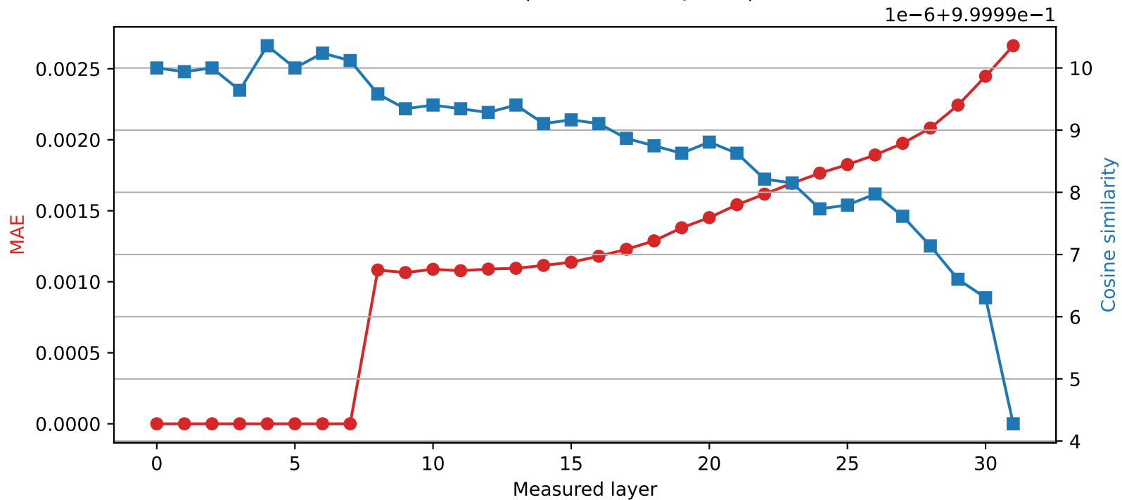
Mistral-7B-Instruct-v0.3 | Quantized layer 7 | float32 → int8
