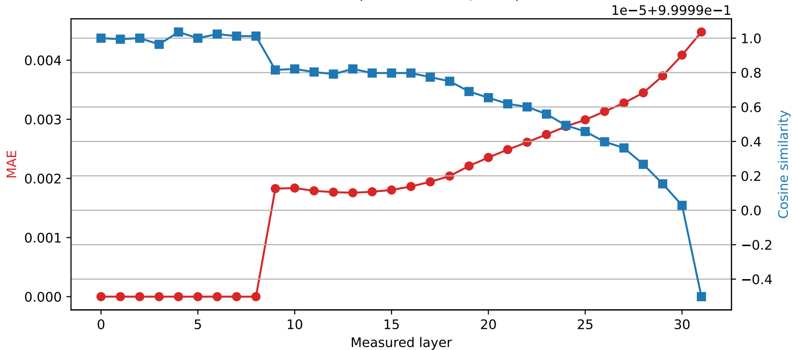
Mistral-7B-Instruct-v0.3 | Quantized layer 8 | float32 → int8
