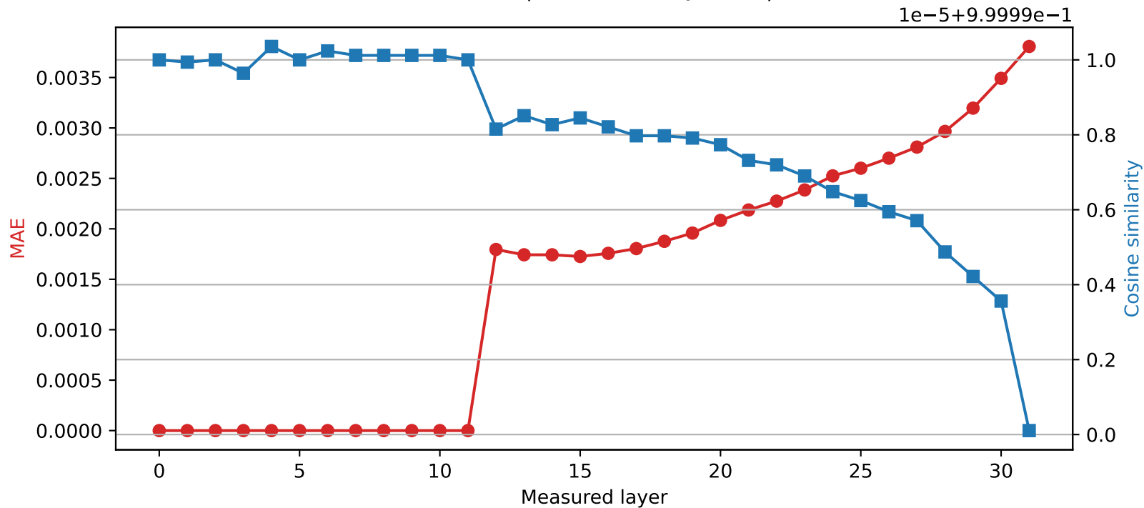
Mistral-7B-Instruct-v0.3 | Quantized layer 11 | float32 \rightarrow int8
