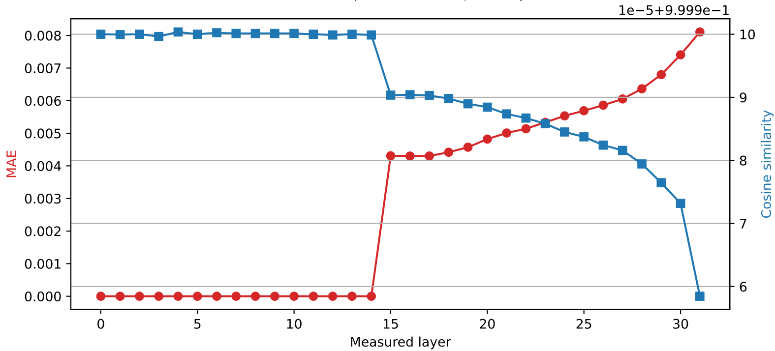
Mistral-7B-Instruct-v0.3 | Quantized layer 14 | float32 \rightarrow int8
