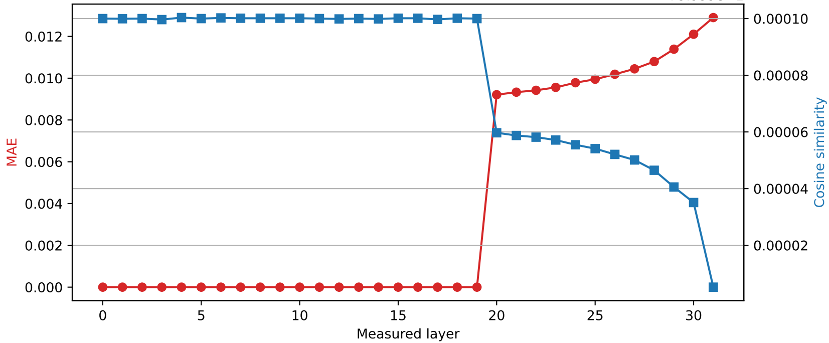
Mistral-7B-Instruct-v0.3 | Quantized layer 19 | float32 \rightarrow int8 +9.999e-1
