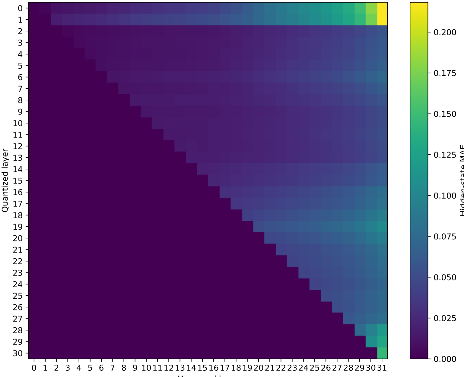
Model: Mistral-7B-Instruct-v0.3 | float32 → int4
