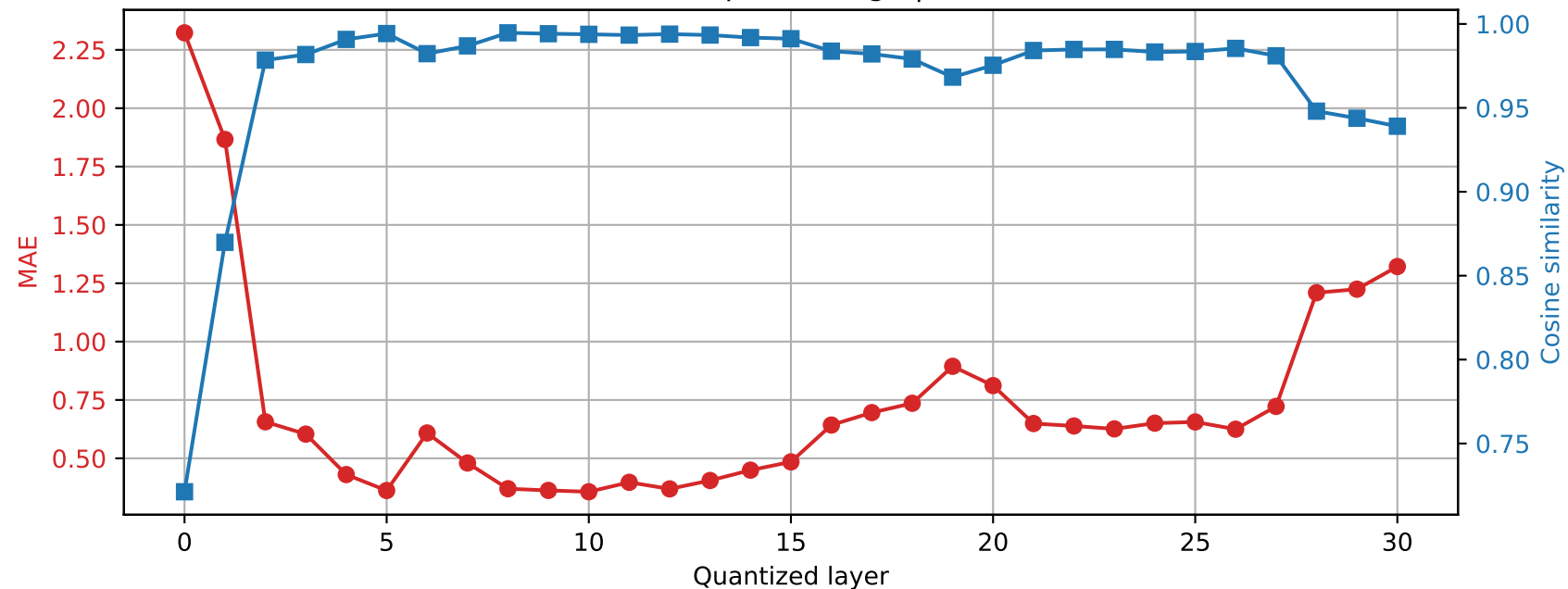
Mistral-7B-Instruct-v0.3 | Prompt 0 Final RMSNorm output damage | float32 → int4
