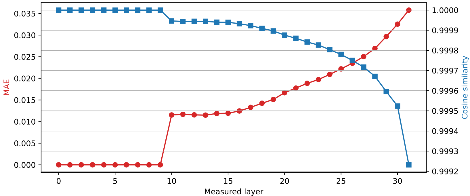
Mistral-7B-Instruct-v0.3 | Quantized layer 9 | float32 → int4
