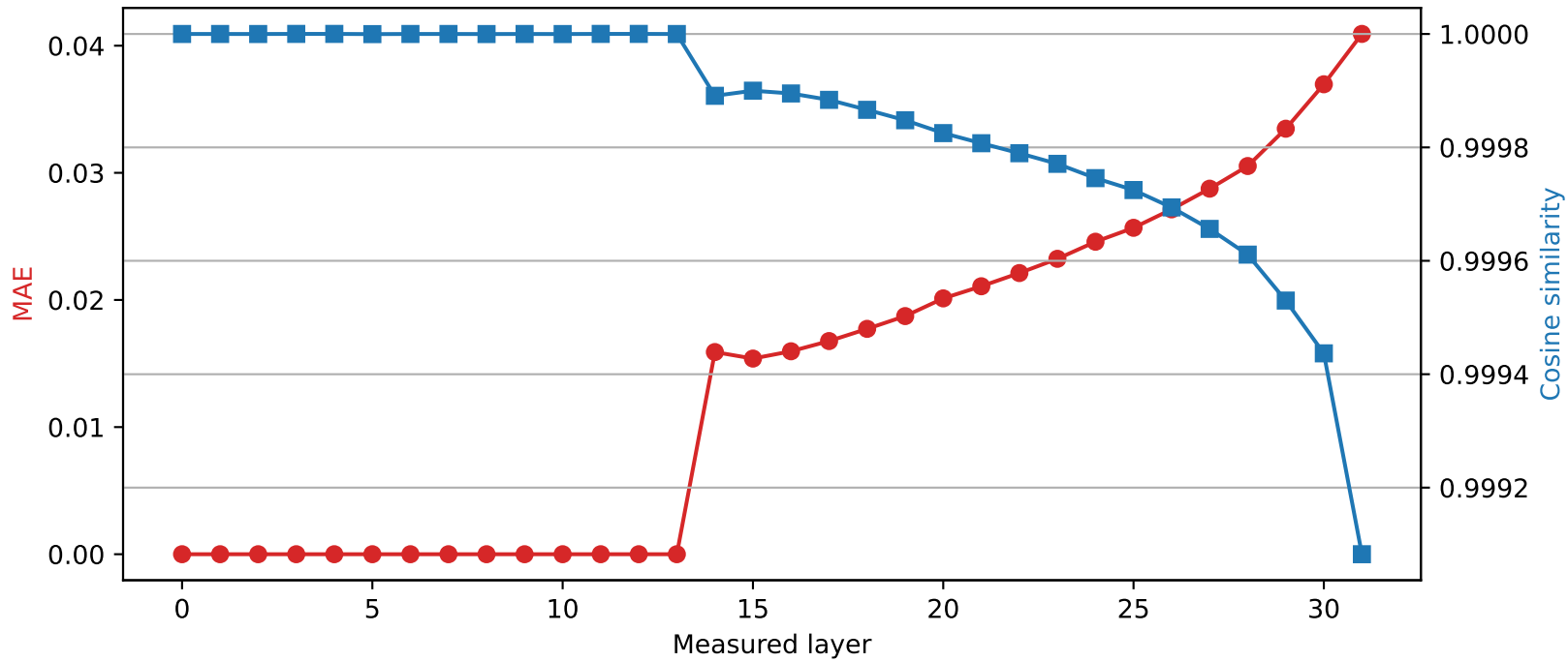
Mistral-7B-Instruct-v0.3 | Quantized layer 13 | float32 \rightarrow int4
