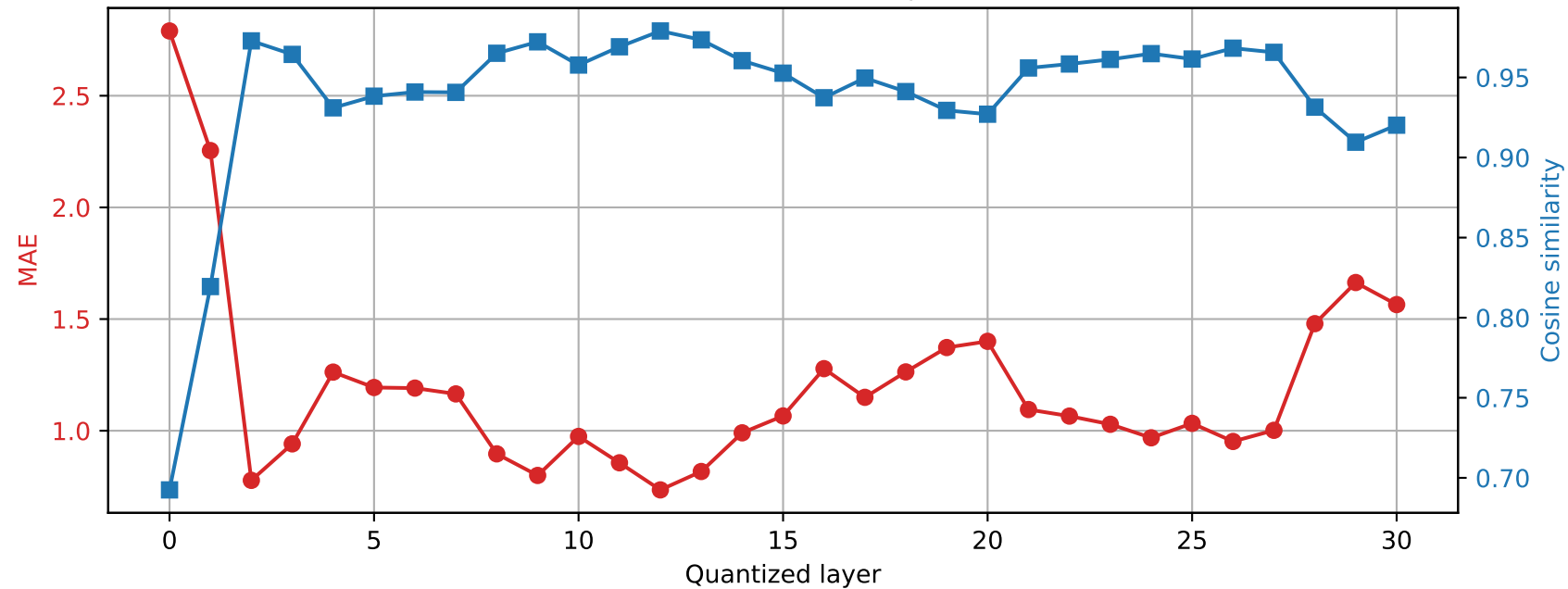
Mistral-7B-Instruct-v0.3 | Prompt 1 Final RMSNorm output damage | float32 → int4
