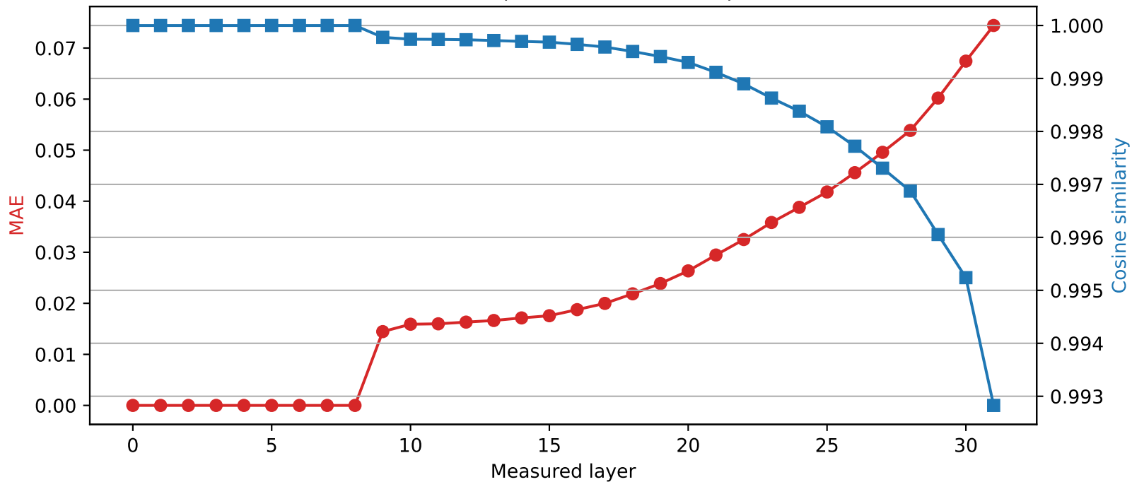
Mistral-7B-Instruct-v0.3 | Quantized layer 8 | float32 → int4
