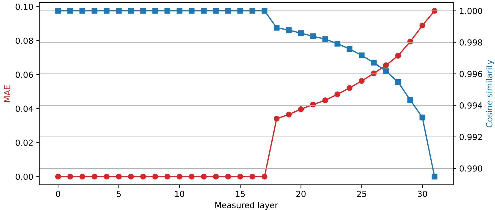
Mistral-7B-Instruct-v0.3 | Quantized layer 17 | float32 \rightarrow int4
