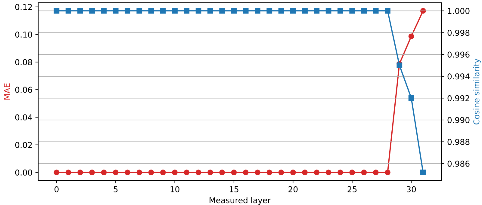
Mistral-7B-Instruct-v0.3 | Quantized layer 28 | float32 \rightarrow int4
