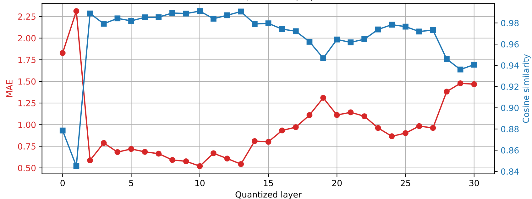
Mistral-7B-Instruct-v0.3 | Prompt 2 Final RMSNorm output damage | float32 \rightarrow int4
