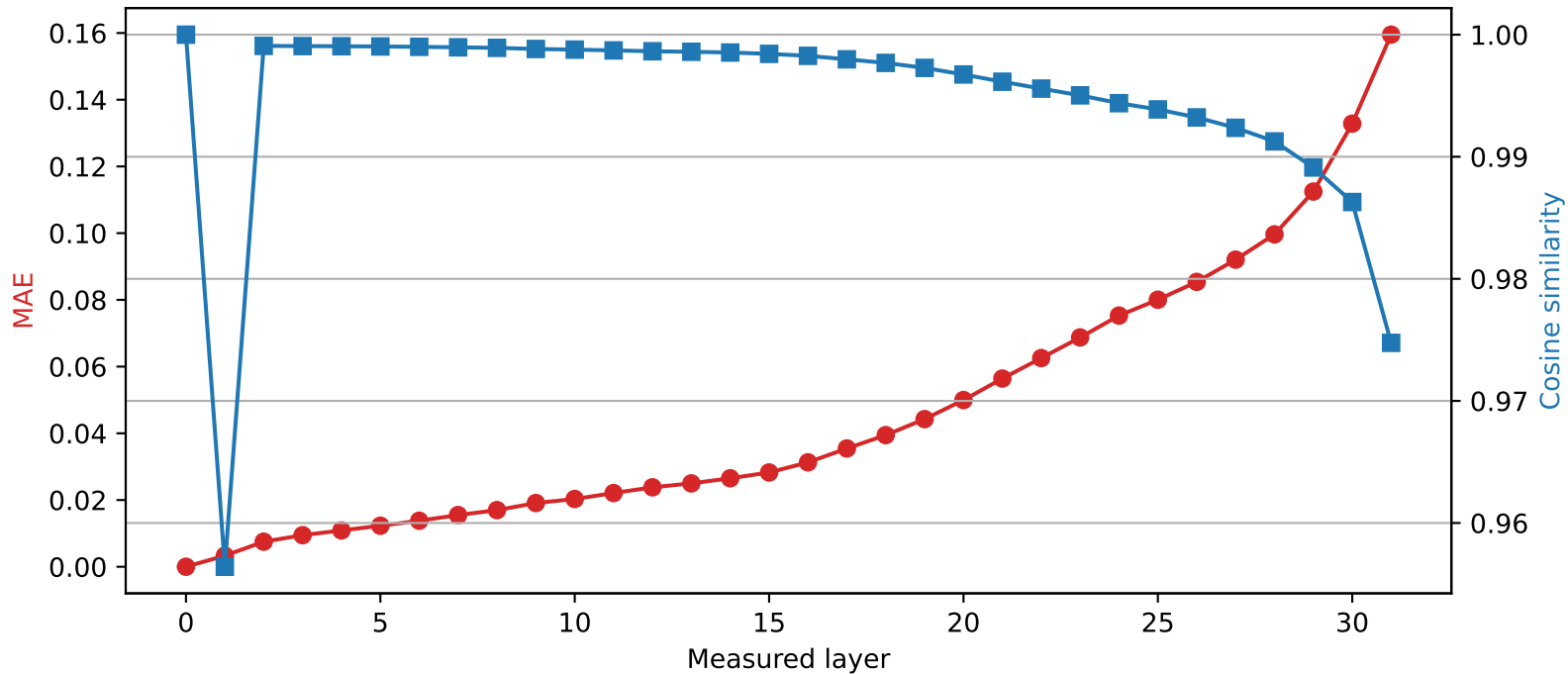
Mistral-7B-Instruct-v0.3 | Quantized layer 0 | float32 \rightarrow int4
