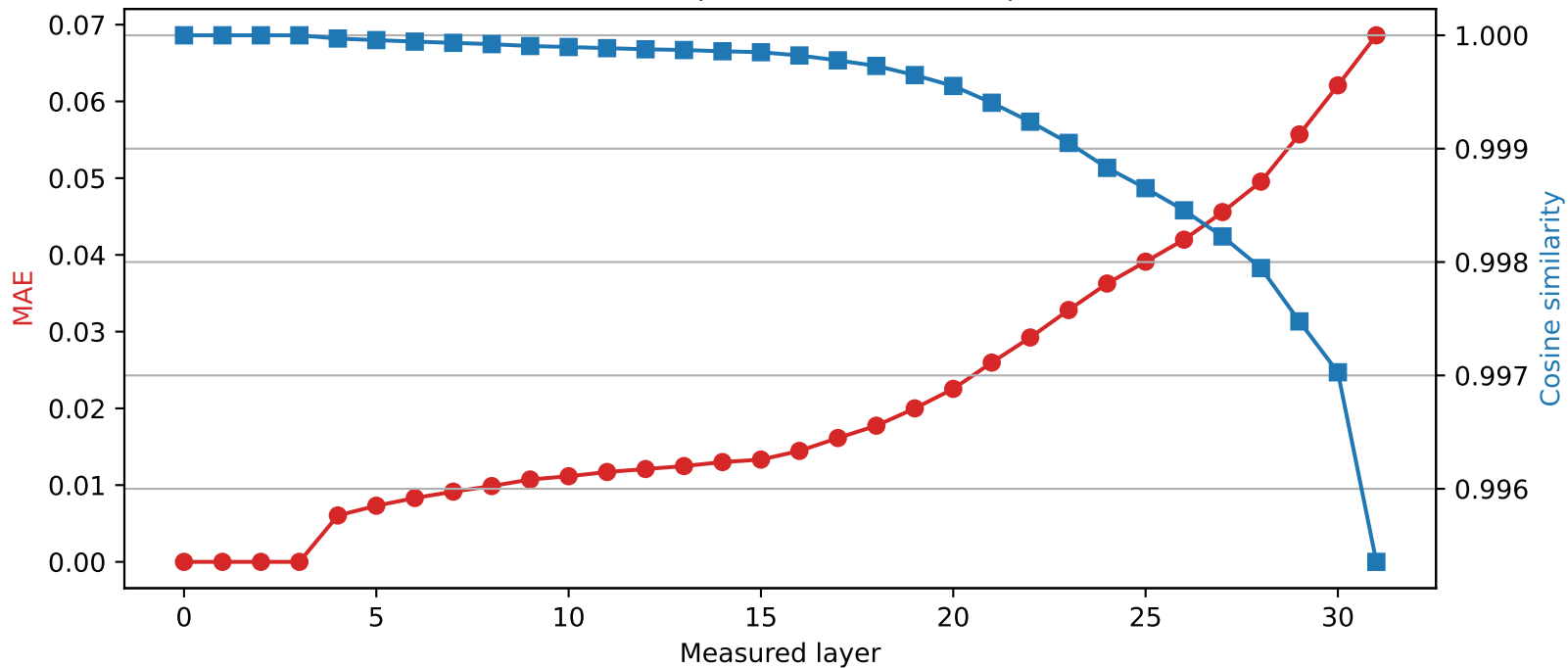
Mistral-7B-Instruct-v0.3 | Quantized layer 3 | float32 \rightarrow int4
