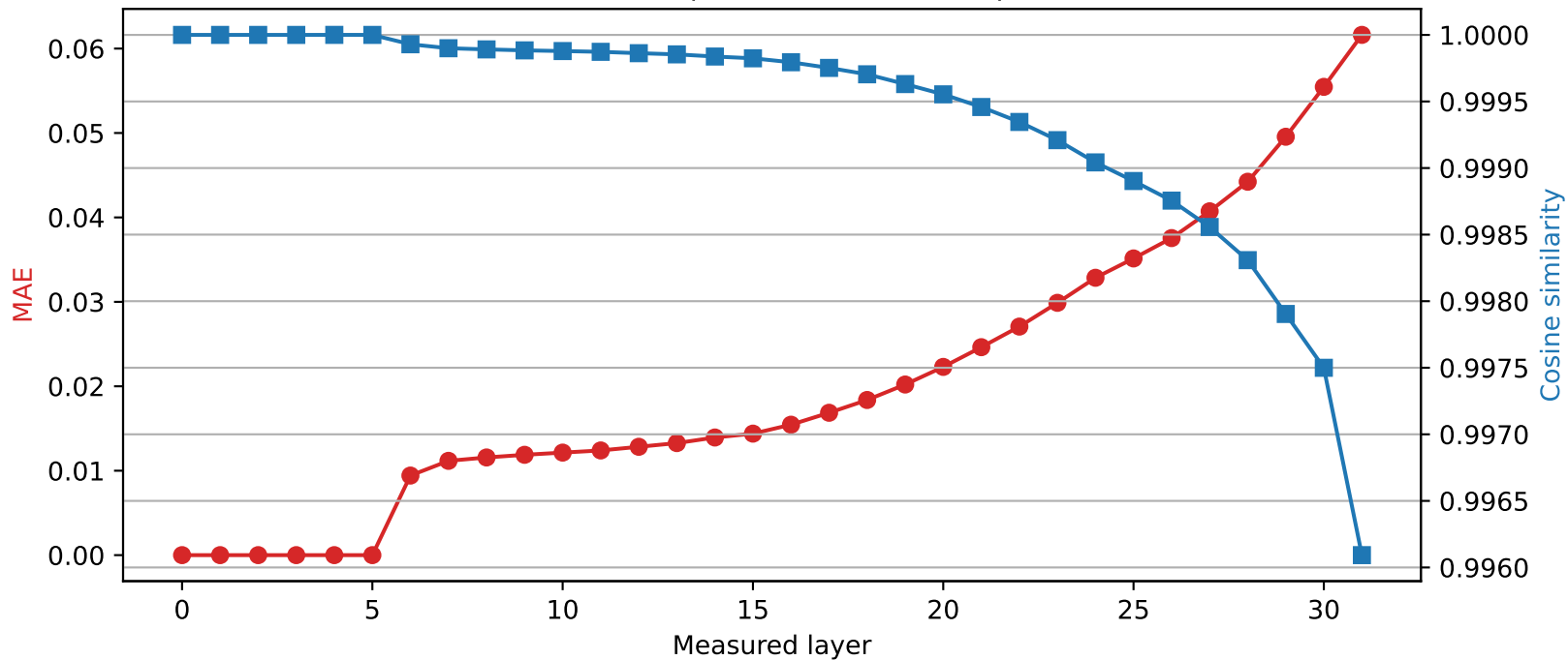
Mistral-7B-Instruct-v0.3 | Quantized layer 5 | float32 \rightarrow int4
