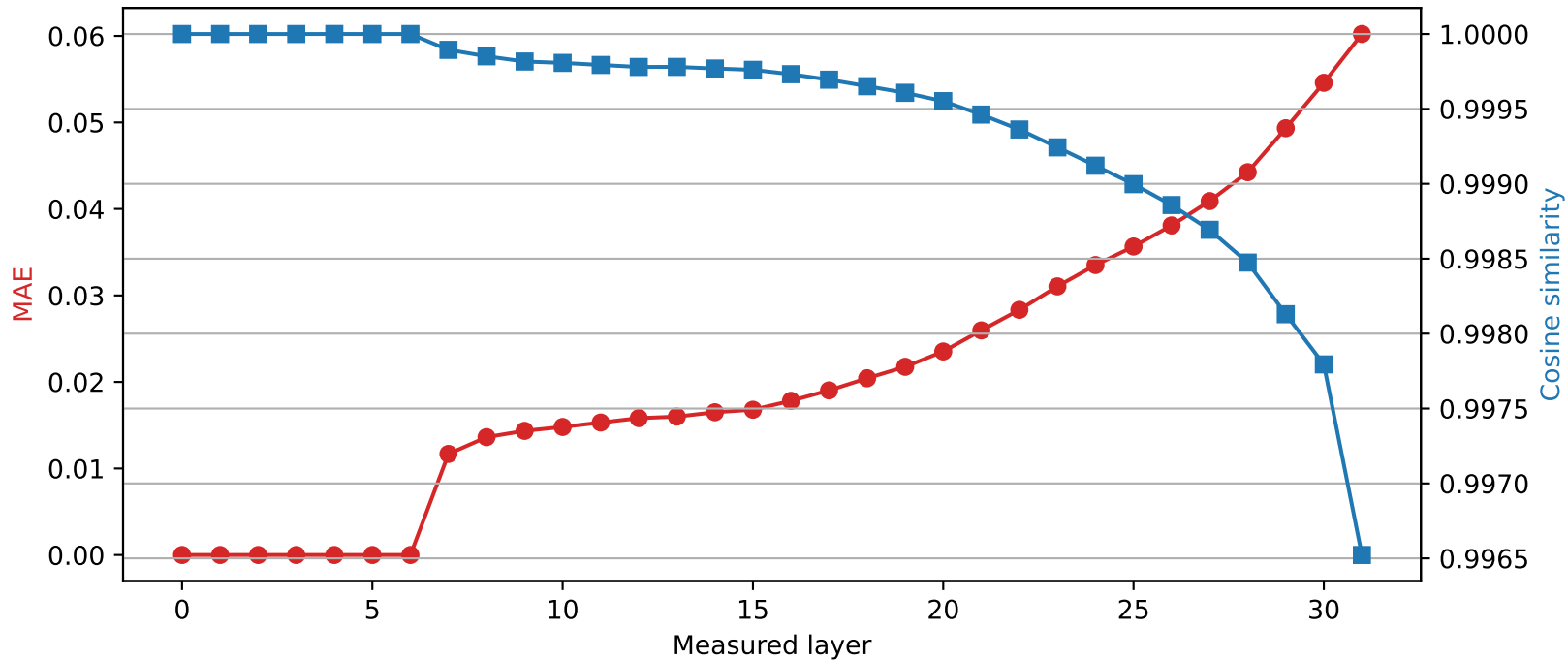
Mistral-7B-Instruct-v0.3 | Quantized layer 6 | float32 \rightarrow int4
