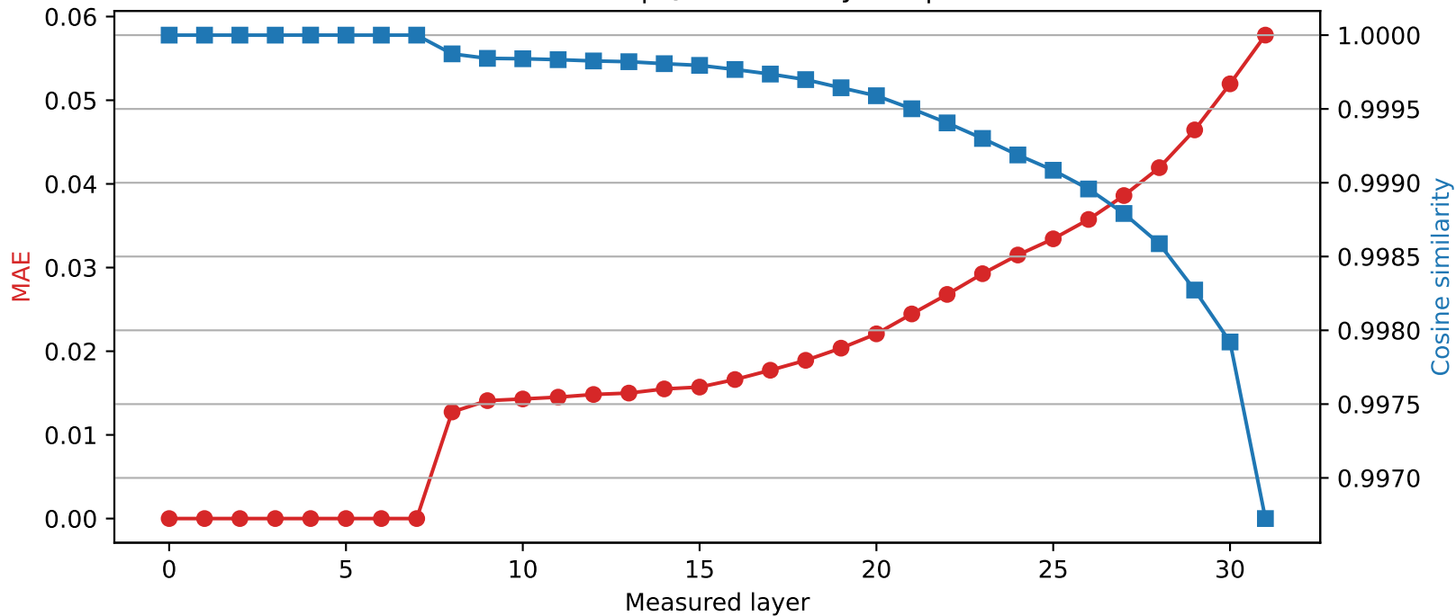
Mistral-7B-Instruct-v0.3 | Quantized layer 7 | float32 \rightarrow int4
