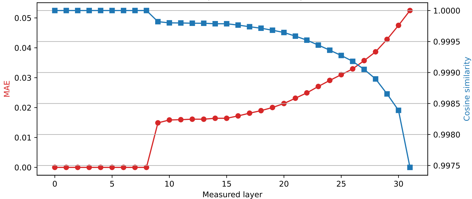
Mistral-7B-Instruct-v0.3 | Quantized layer 8 | float32 \rightarrow int4
