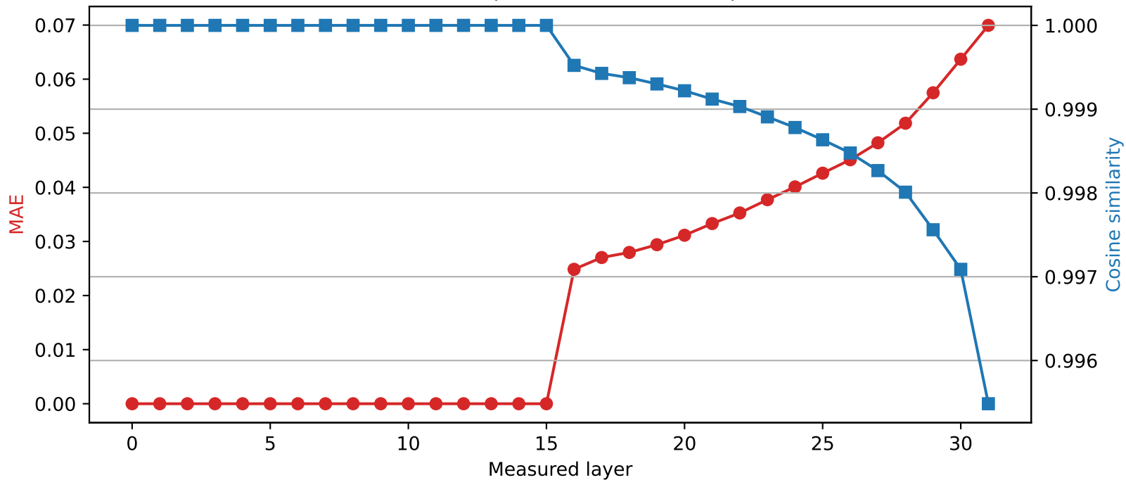
Mistral-7B-Instruct-v0.3 | Quantized layer 15 | float32 \rightarrow int4
