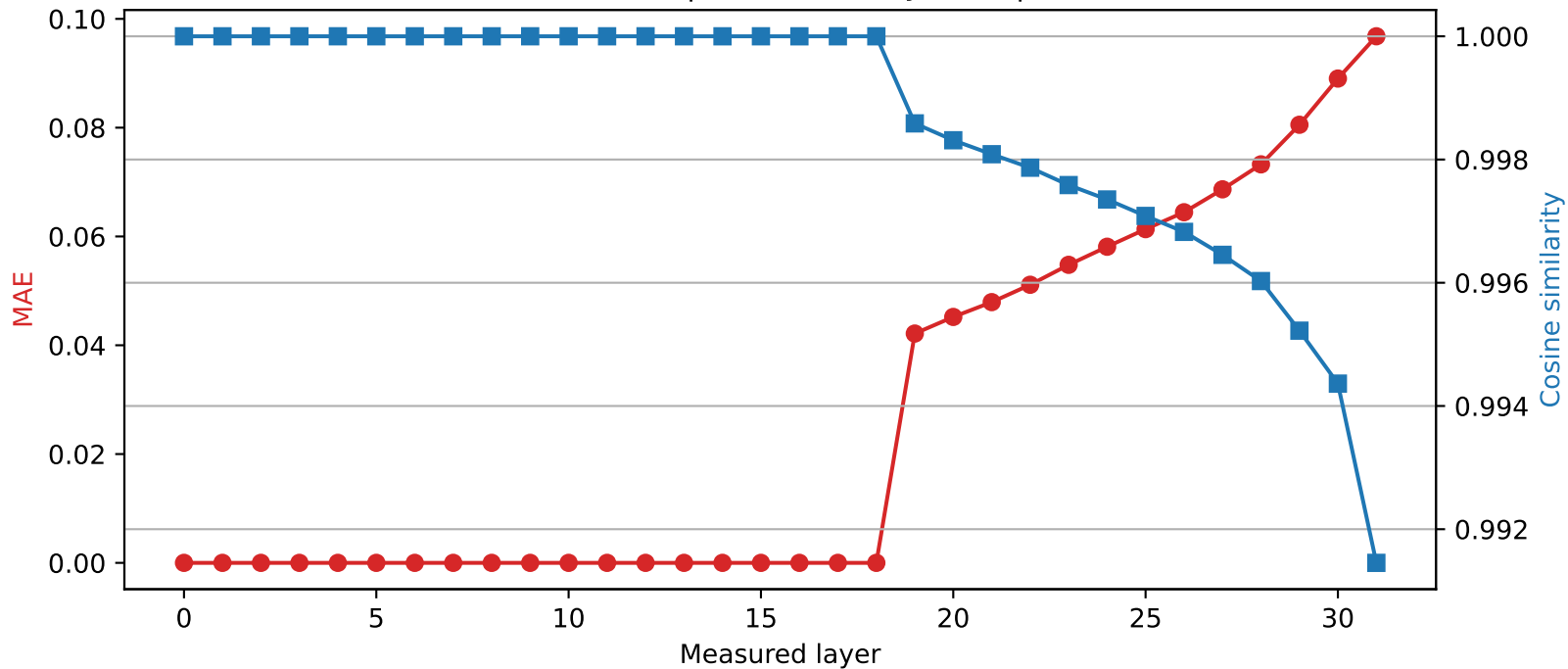
Mistral-7B-Instruct-v0.3 | Quantized layer 18 | float32 \rightarrow int4
