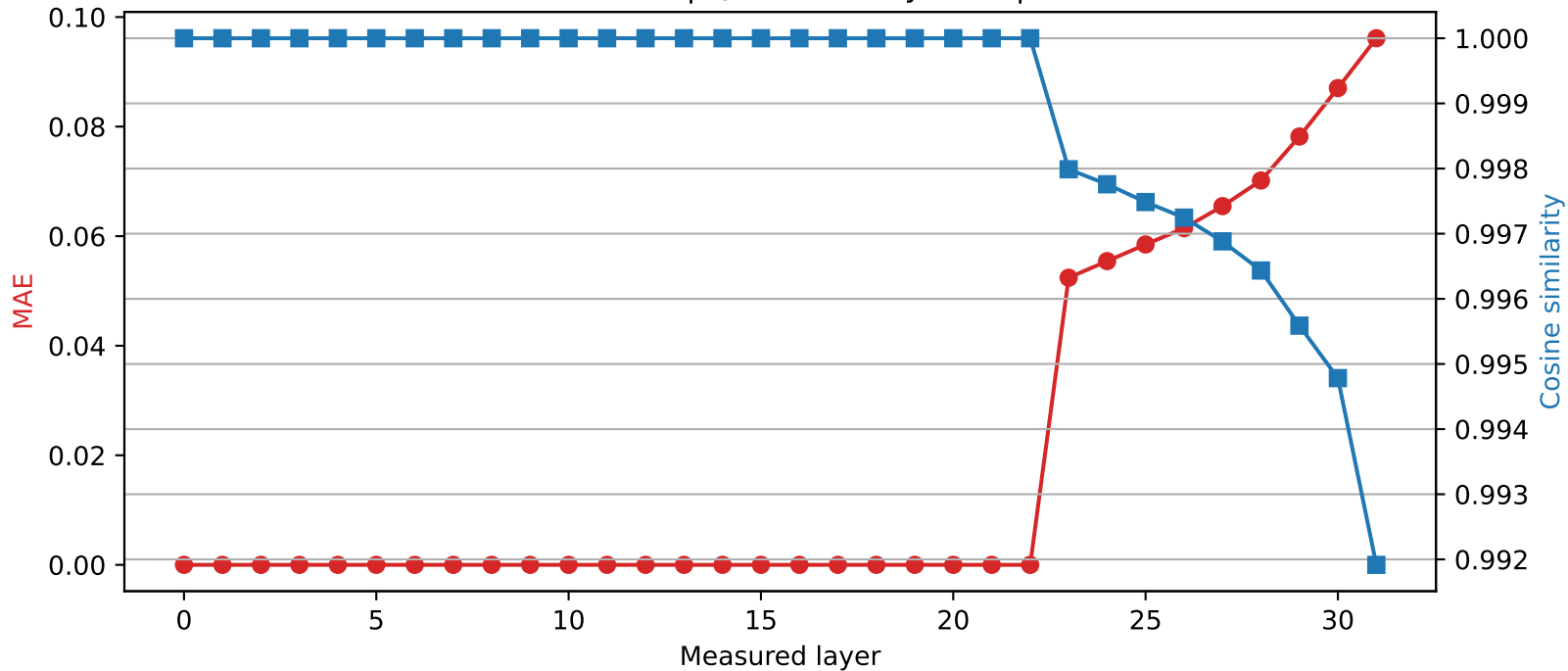
Mistral-7B-Instruct-v0.3 | Quantized layer 22 | float32 \rightarrow int4
