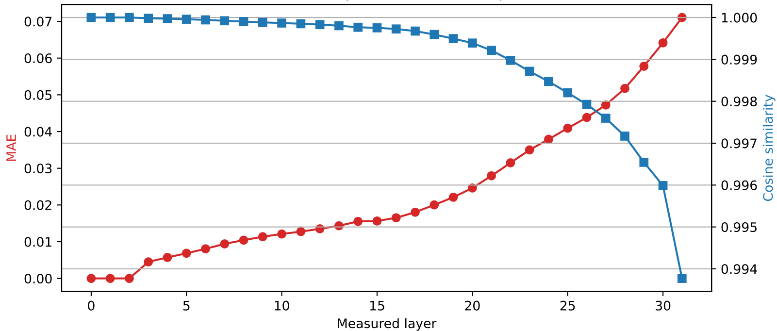
Mistral-7B-Instruct-v0.3 | Quantized layer 2 | float32 \rightarrow int4
