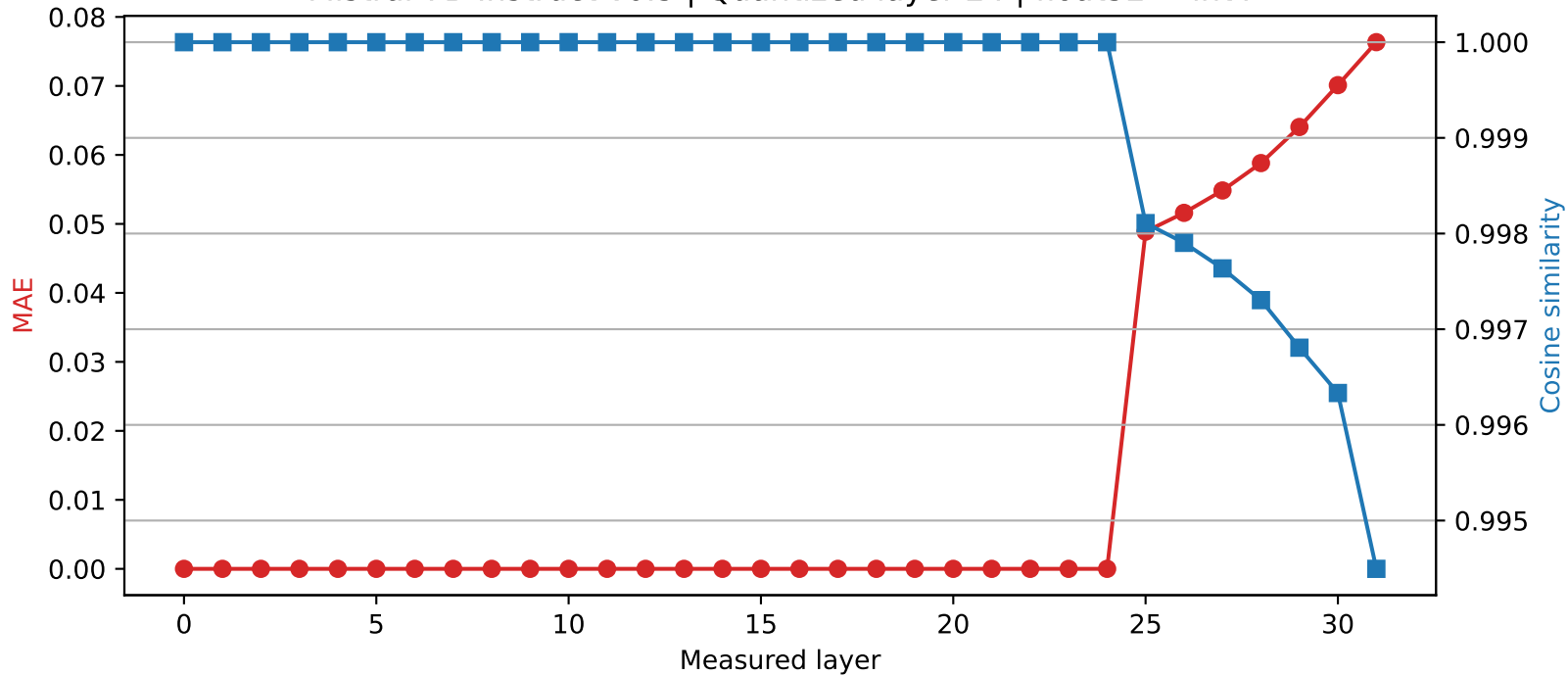
Mistral-7B-Instruct-v0.3 | Quantized layer 24 | float32 \rightarrow int4
