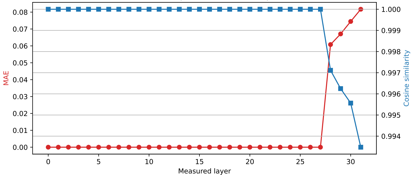
Mistral-7B-Instruct-v0.3 | Quantized layer 27 | float32 \rightarrow int4
