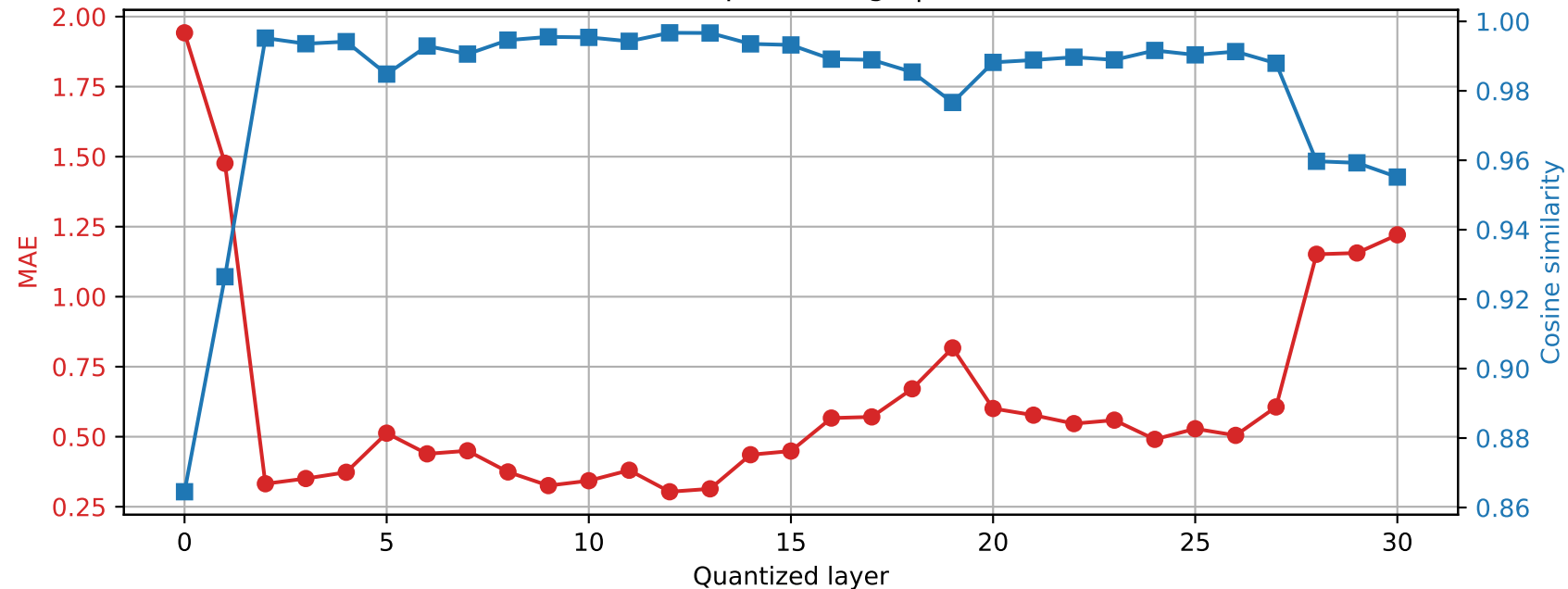
Mistral-7B-Instruct-v0.3 | Prompt 4 Final RMSNorm output damage | float32 \rightarrow int4
