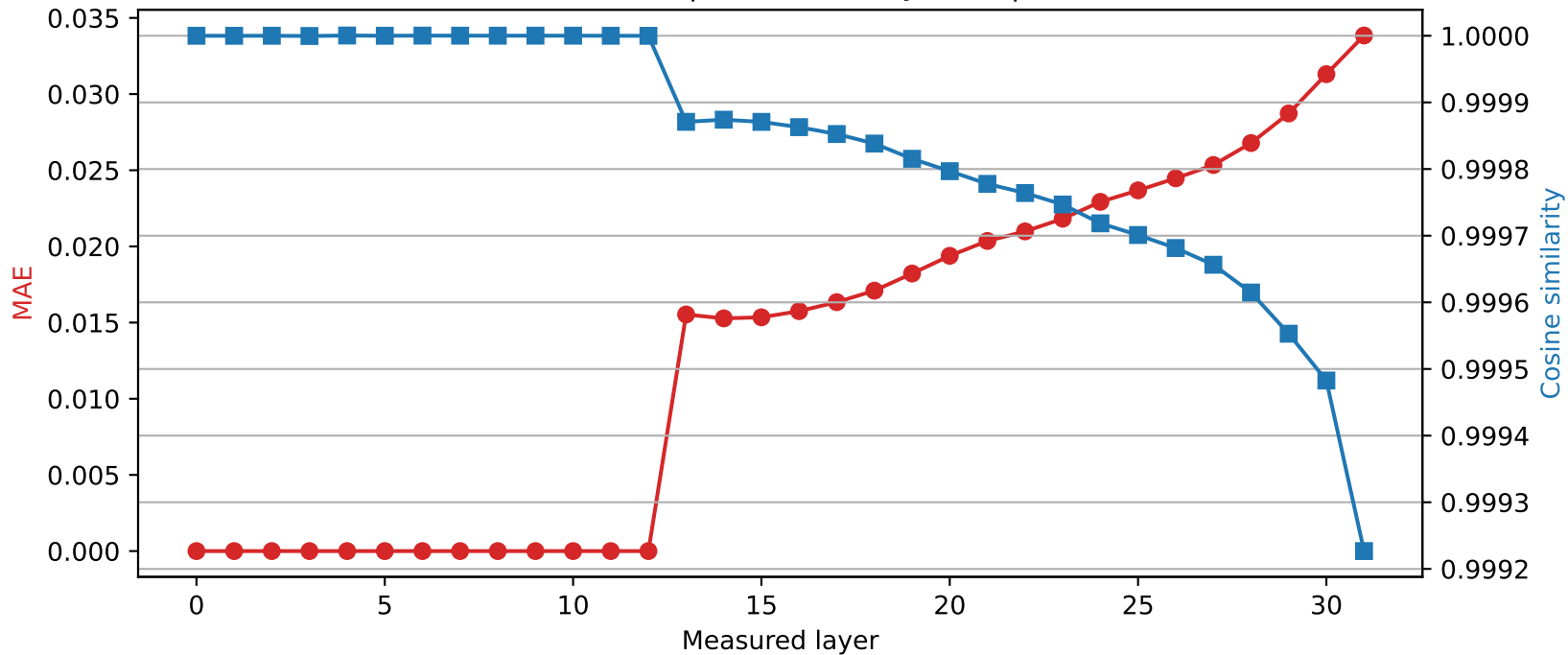
Mistral-7B-Instruct-v0.3 | Quantized layer 12 | float32 \rightarrow int4
