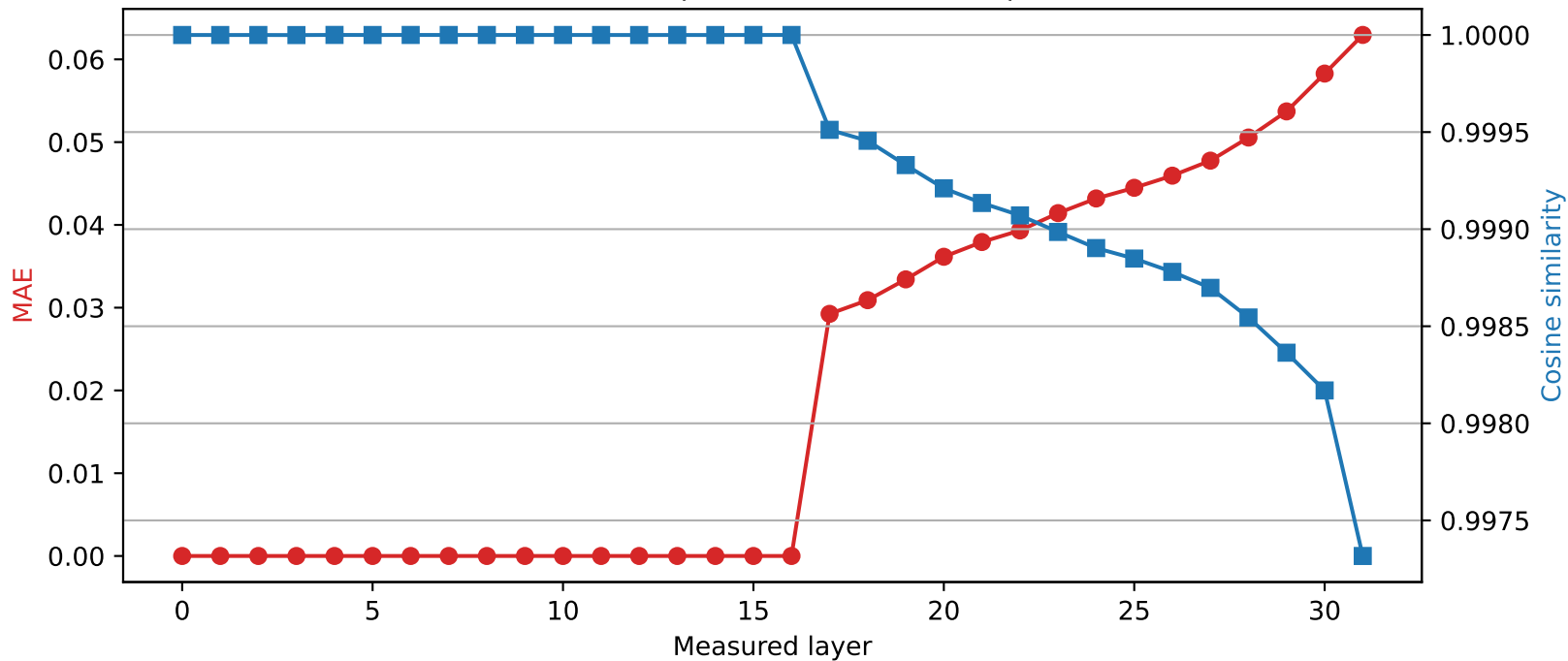
Mistral-7B-Instruct-v0.3 | Quantized layer 16 | float32 \rightarrow int4
